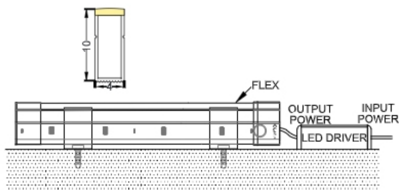
Clamp Mounted
