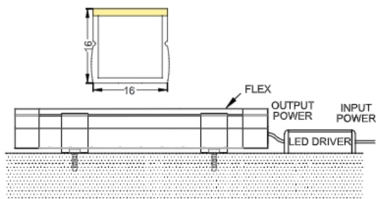
Clamp Mounted
