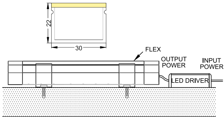
Clamp Mounted
