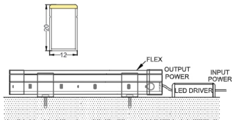
Clamp Mounted
