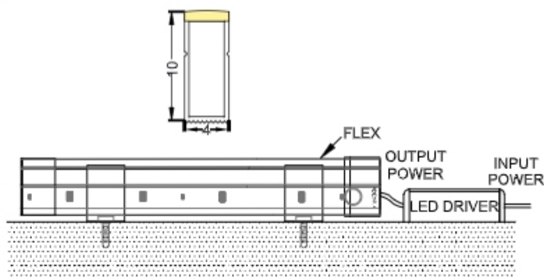
Clamp Mounted
