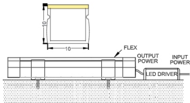
Clamp Mounted
